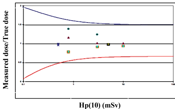
— upper limit for photon — lower limit for photon × S-Cs ▲ S-Cs rot ● w-250 rot ■ S-Cs & w-80 ■ S-Cs & w-80 rot
